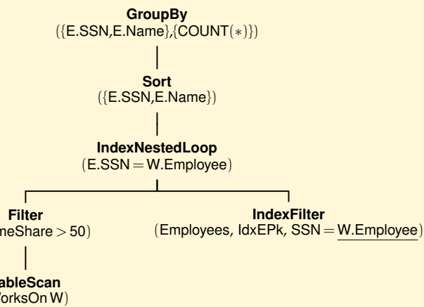
Physical query plan with indexes
