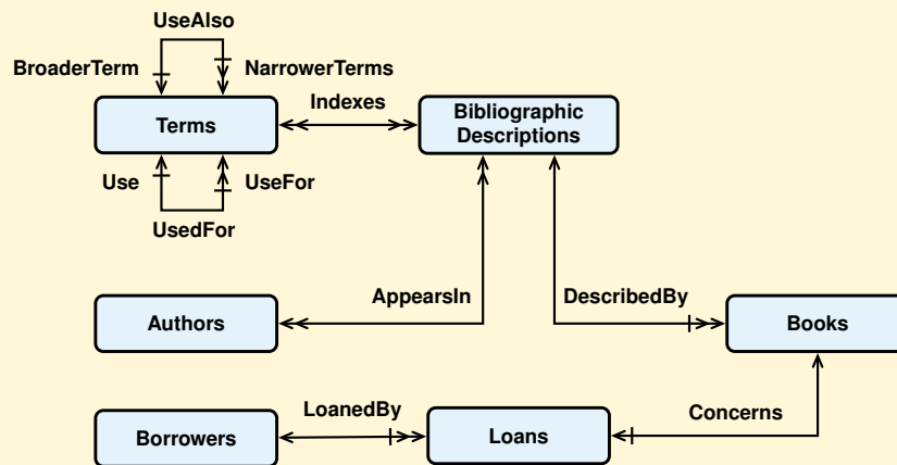
Figure 2.4: An initial conceptual schema for a library
